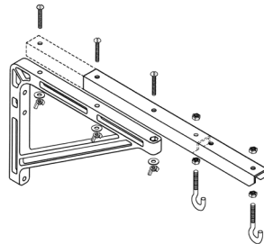
No. 23 Adjustable Wall Bracket Screen can be extended 10", 14", 15 3/4", 18 3/4", 20" or 24" from wall by wing nut and bolt adjustment.
